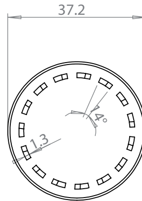
inner cap
