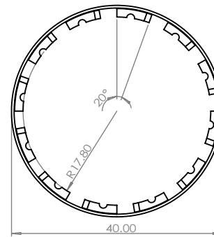
inner cap
