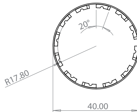
inner cap
